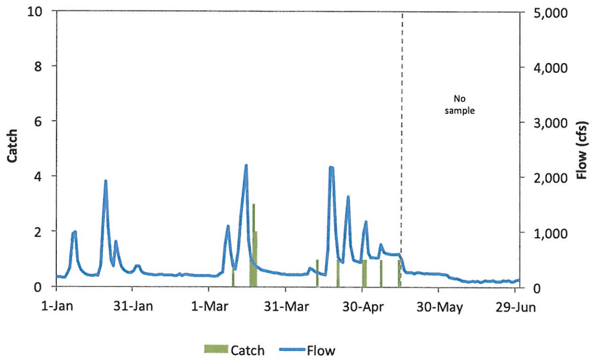
Figure 3. Grayson Chinook catch and Tuolumne River flow at Modesto, 2016.
