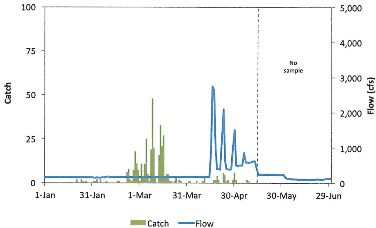
Figure 1. Waterford Chinook catch and Tuolumne River flow at La Grange, 2016.
