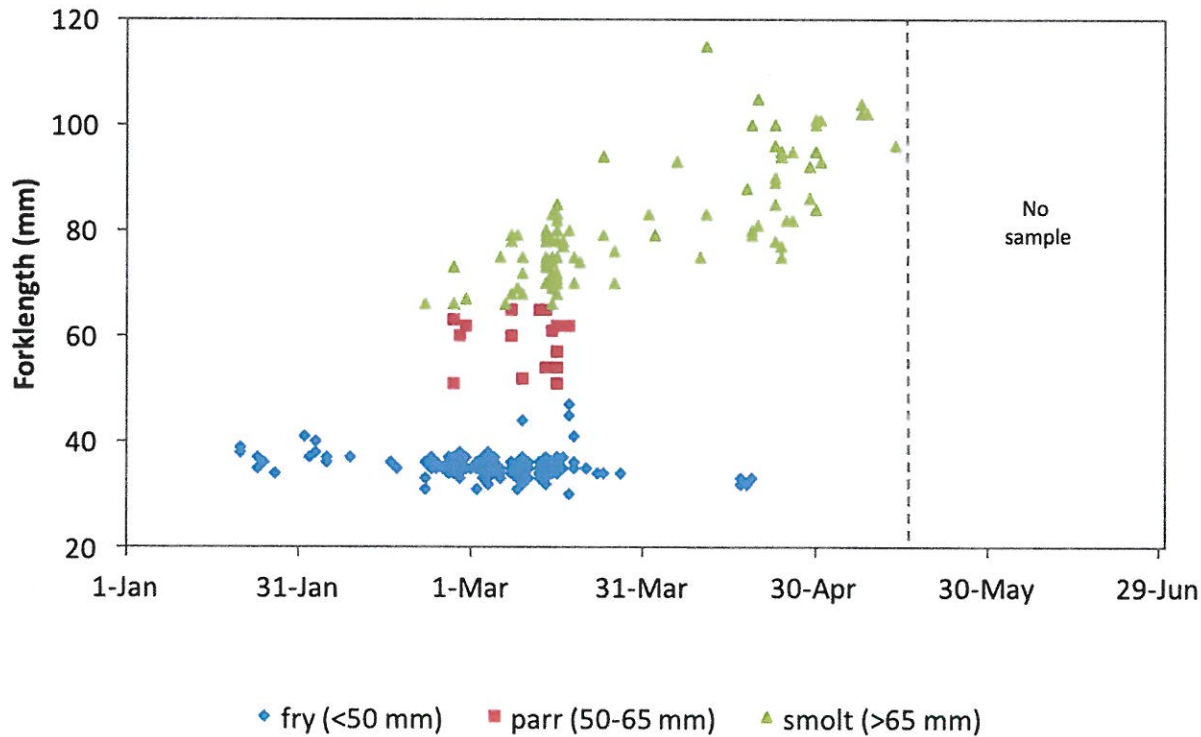
Figure 2. Chinook forklength by lifestage at Waterford, 2016.
