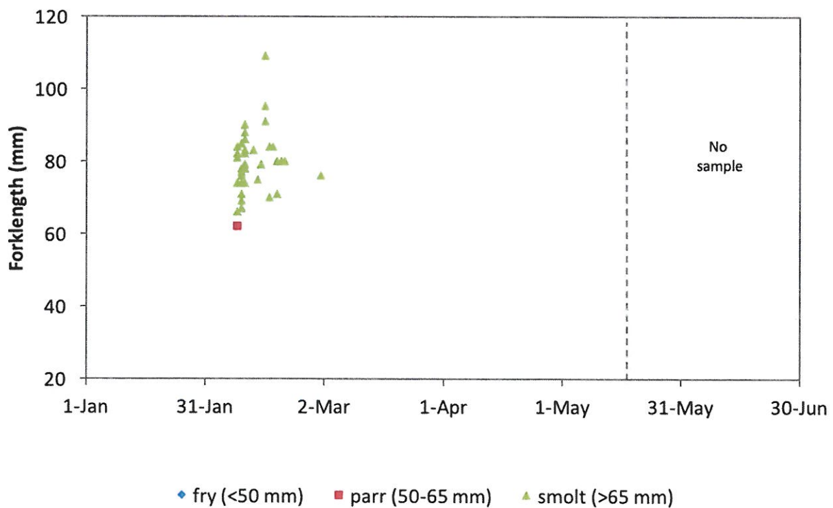
Figure 4. Chinook forklength by lifestage at Grayson, 2016.
